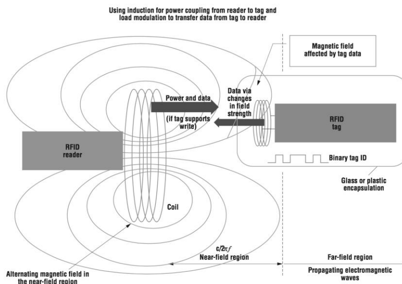
FIGURE 2: NEAR-FIELD COUPLING (WANT 2006)
