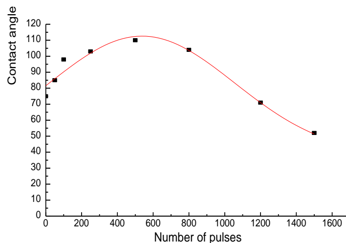
FIGURE 4. THE CONTACT ANGLE OF WATER VERSUS THE NUMBER OF LASER PULSES FOR PET POLYMER AT THE FLUENCE OF 50 \text{ mJ/cm}^2 .
