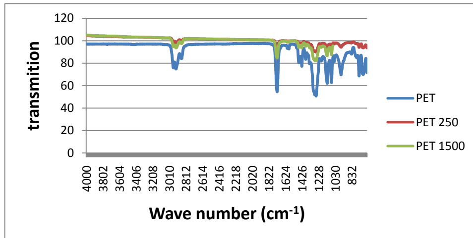
FIGURE 3. FTIR SPECTRUM OF UNTREATED AND IRRADIATION SAMPLE OF A PET POLYMER AT 50 \text{ mJ/cm}^2 with 250 and 1500 pulses.
