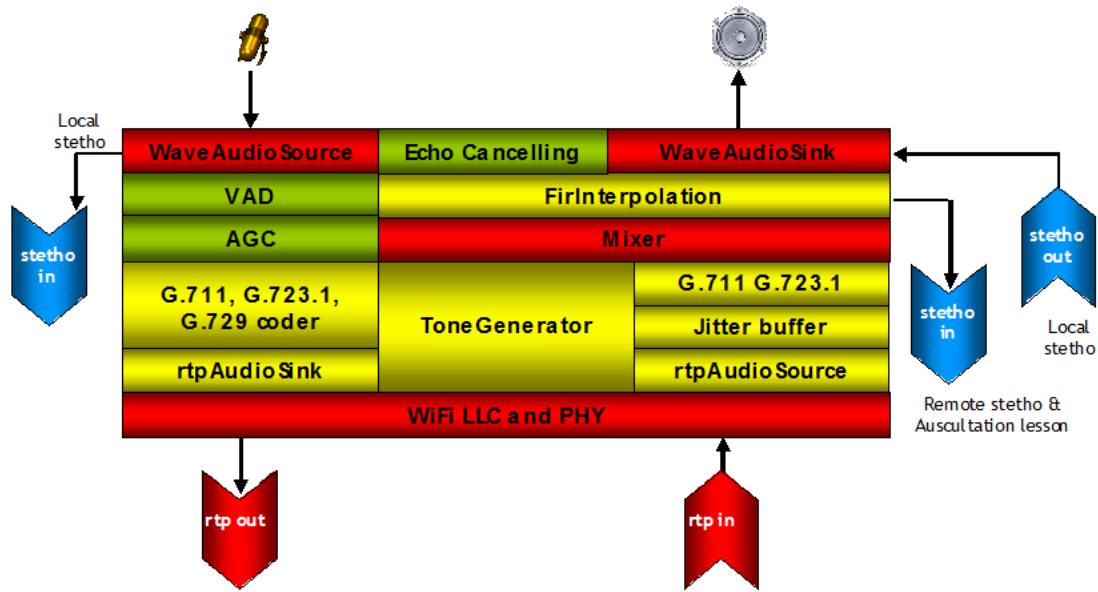
FIGURE 14: SOFTPHONE (MPC) ARCHITECTURE
