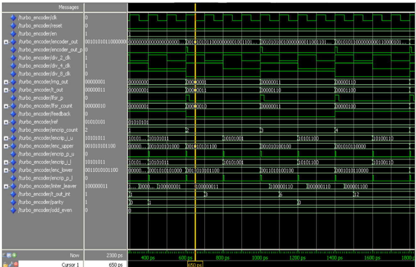
FIG.14 OUTPUT WAVEFORM OF TURBO ENCODER.
