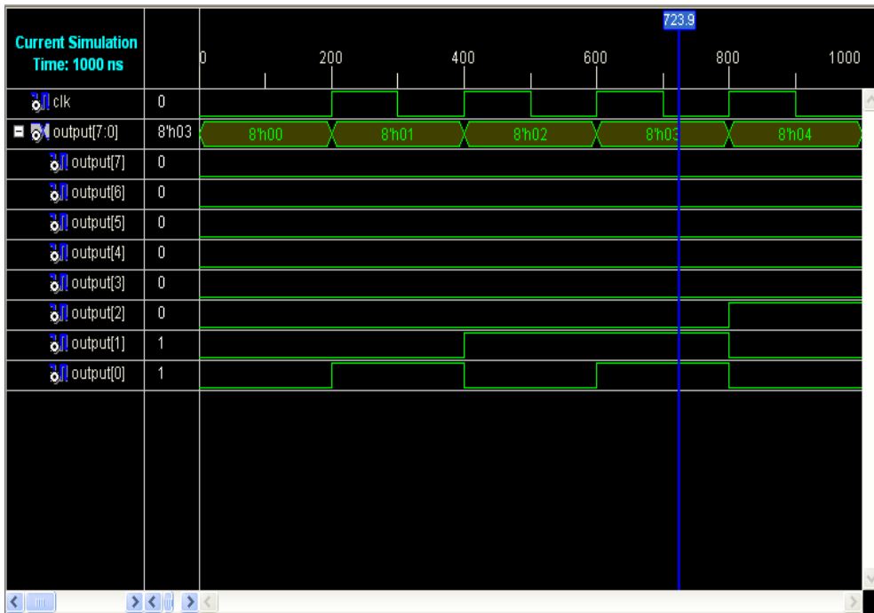
FIG.12 WAVEFORM OF COUNTER.
