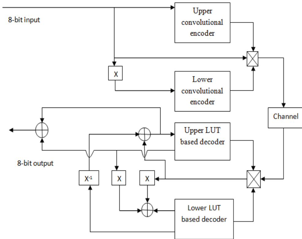
FIG.1 TURBO ENCODER AND DECODER SCHEME.
