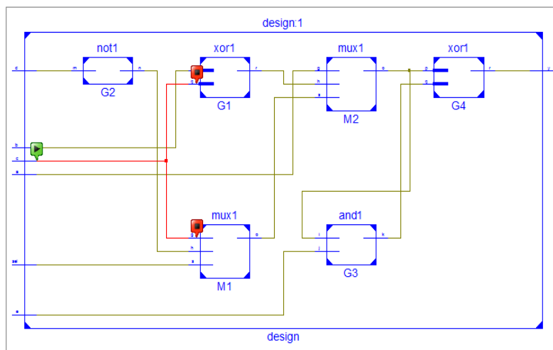
FIG.15 RTL SCHEMATIC OF ACS BLOCK.
