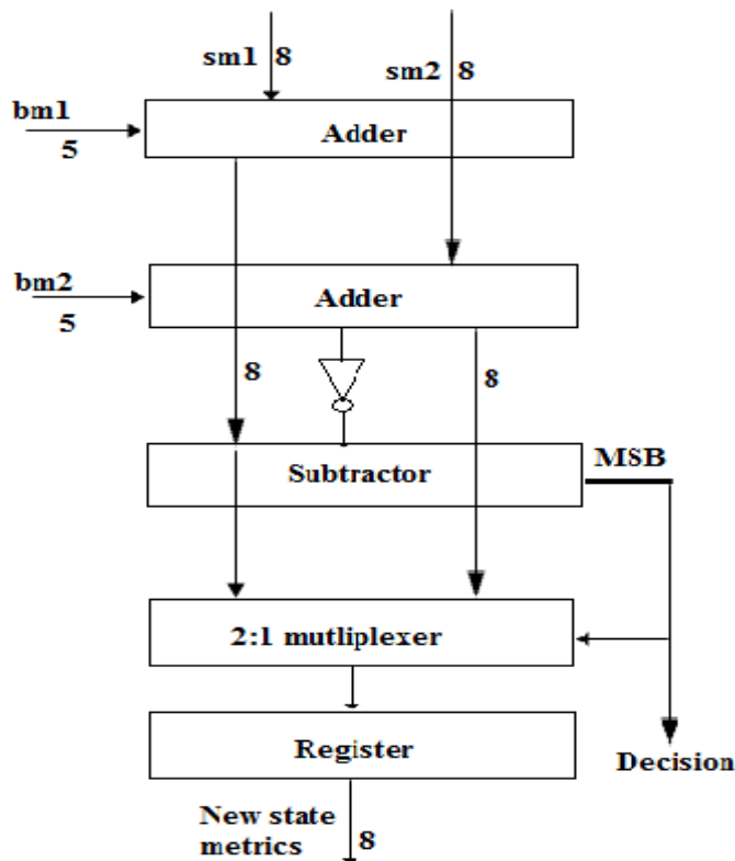
FIG.6 ACS UNIT
