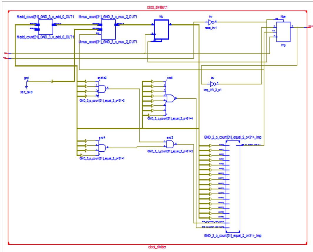
FIG.9 RTL SCHEMATIC OF CLOCK DIVIDER.
