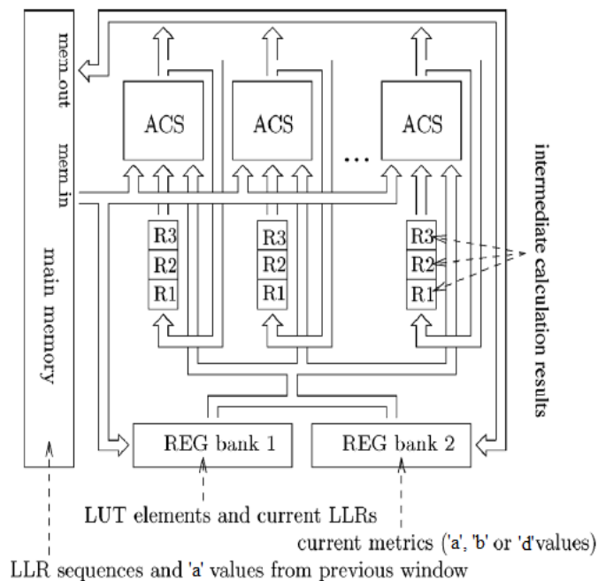
FIG.5 ENERGY-EFFICIENT LOOKUP TABLE ARCHITECTURE
