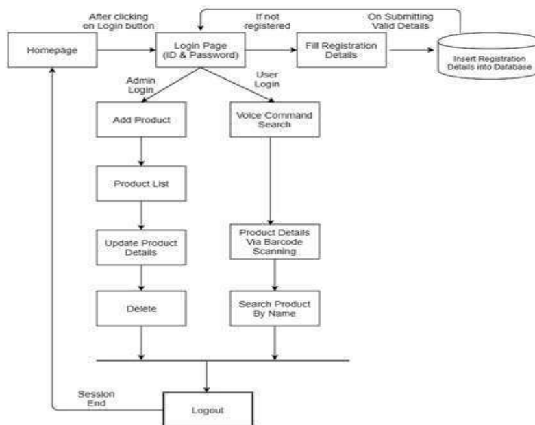
Figure (3): System Architecture
