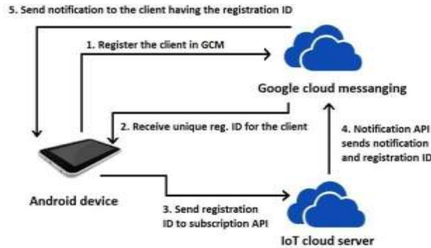
Fig. 4: Functional block diagram of android application
