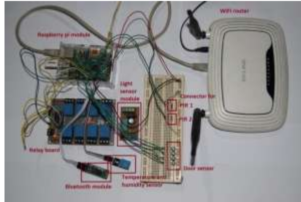
Fig. 6: Experimental setup
