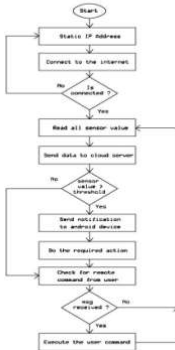
Fig. 5: Flowchart of home automation controller device
