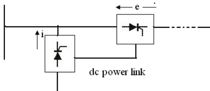
Fig.5 Structure of Combined Series-Shunt Controllers
