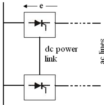
Fig.4 Structure of Combined Series-Series Controllers
