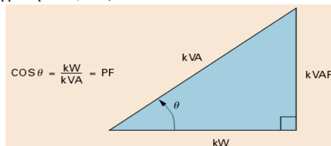
Fig.1 Structure of Power Triangle
