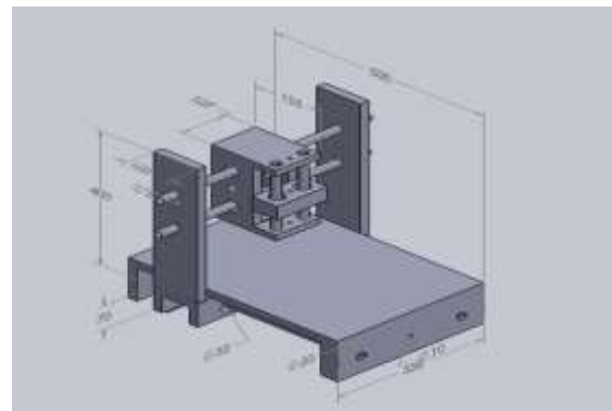
Fig. 5 Solid Model Design
