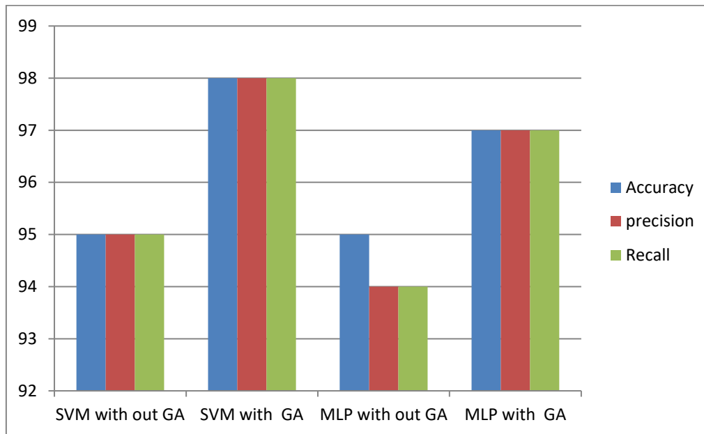
Figure-4: Performance of Classifier Multi-Label Classification
