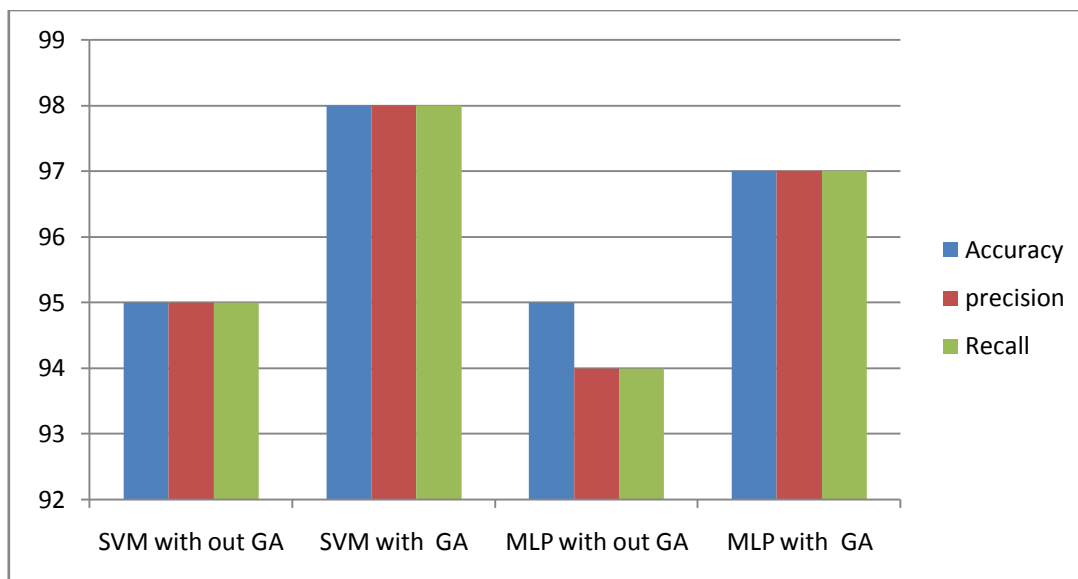
FIGURE 4: Performance of Classifier Multi- Label Classification
