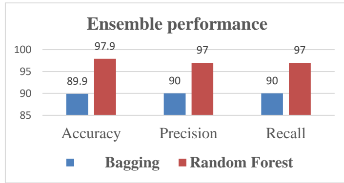
Figure-3: Performance of Ensemble classifiers
