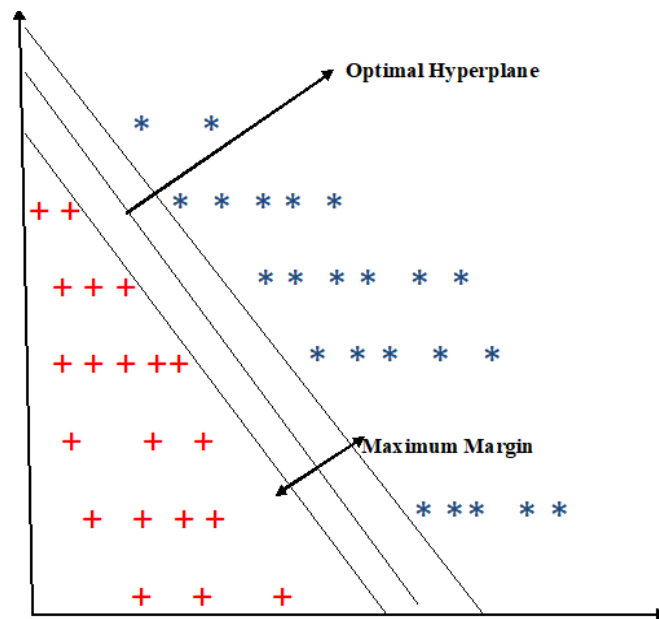
FIGURE 1: Optimal Hyperplane
