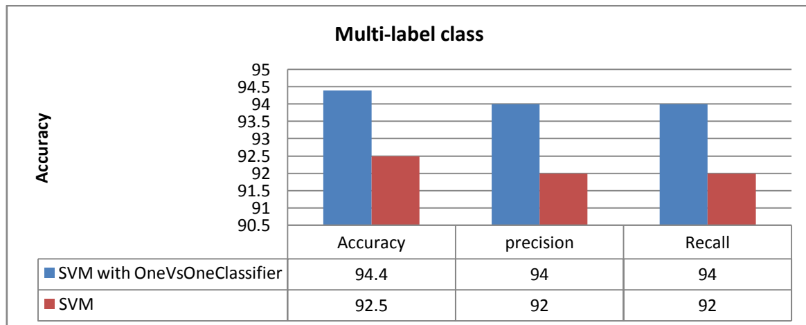
FIGURE 5: Performance of SVM with OneVsOne Classifier Multi- Label Classification
