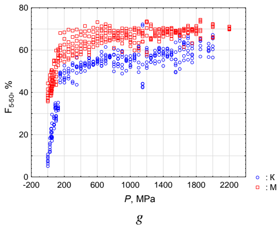
FIG. 2. CHANGE OF FRACTIONAL COMPOSITION OF MONTMORILLONITE (M) AND KAOLINITE (K) OF NATURAL CLAYS UNDER PRESSURE. FRACTIONS: a - F_{<0,1} , b - F_{0,1-0,2} , c - F_{0,2-0,5} , d - F_{0,5-1} , e - F_{1-2} , f - F_{2-5} , f - F_{5-50}
