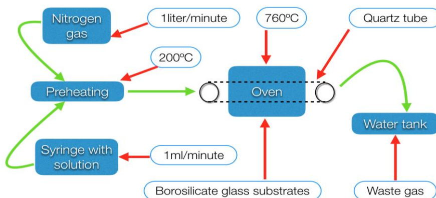
FIG. 1. The spray pyrolysis system.
