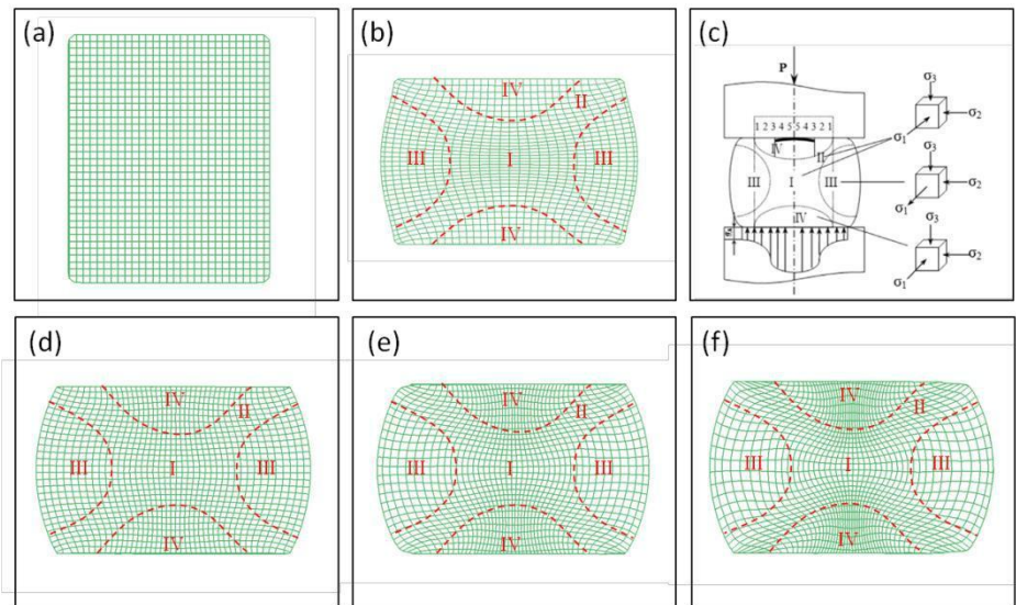
FIGURE 5: CROSS SECTIONS OF THE SIMULATED FLOW LINES OF 2A14 ALUMINUM ALLOYS PROCESSED BY MDF UNDER VARIOUS CUMULATIVE STRAINS: (a) \Sigma\Delta\varepsilon=0 ; (b) \Sigma\Delta\varepsilon=0.4 ; (c) SCHEMATIC DIAGRAM OF FOUR DEFORMATION ZONES DURING MDF; (d) \Sigma\Delta\varepsilon=1.2 ; (e) \Sigma\Delta\varepsilon=2.4 (f) \Sigma\Delta\varepsilon=3.6
