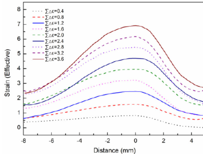
FIGURE 8: RELATIONSHIP BETWEEN EFFECTIVE STRAIN AND THE DISTANCE FROM THE EDGE OF THE DRUM SHAPE (POINT -P) TO THE CENTER (POINT O), THEN TO THE CONTACT SURFACE (POINT P)
