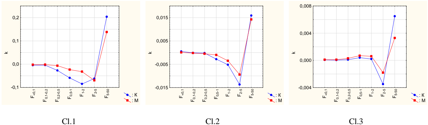
Cl.1 Cl.2 Cl.3 FIG. 3. DEPENDENCE OF PRESSURE EFFECT DEGREE ON CHANGING OF INVESTIGATED FRACTION CONTENTS FOR KAOLINITE AND MONTMORILLONITE NATURAL CLAYS REFERRING TO CLASSES 1, 2 AND 3
