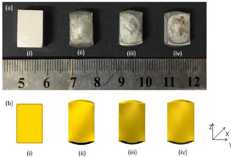
FIGURE 4 APPEARANCES OF THE 2A14 ALUMINUM ALLOY BILLETS DURING MDF OBTAINED BY (a) EXPERIMENTS AND (b) FEM: (i) BEFORE MDF; (ii) \sum\Delta \epsilon=1.2 ; (iii) \sum\Delta \epsilon=2.4 ; (iv) \sum\Delta \epsilon=3.6
